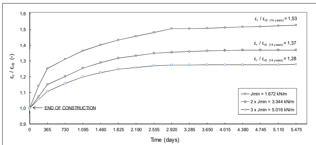
Figure 4. Influence of reinforcement stiffness on relative evolution of mobilized reinforcement strains with time.
