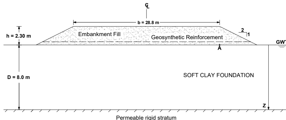
Figure 1. Considered embankment geometry and foundation soil stratigraphy.
