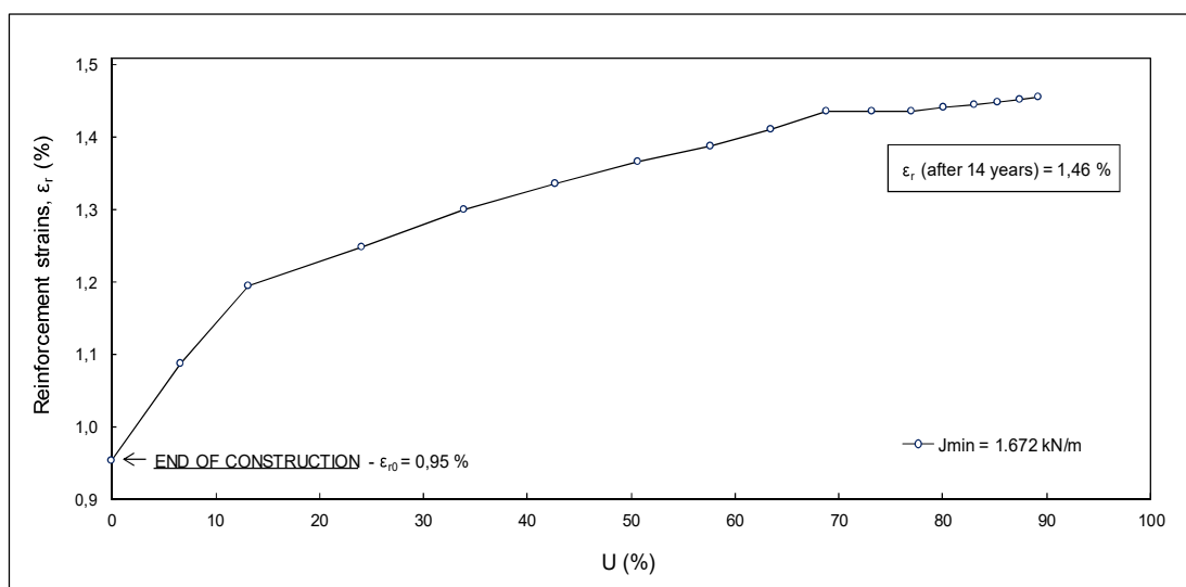
Figure 2. Mobilized reinforcement strains along the dissipation of the excess of pore-water pressures.
