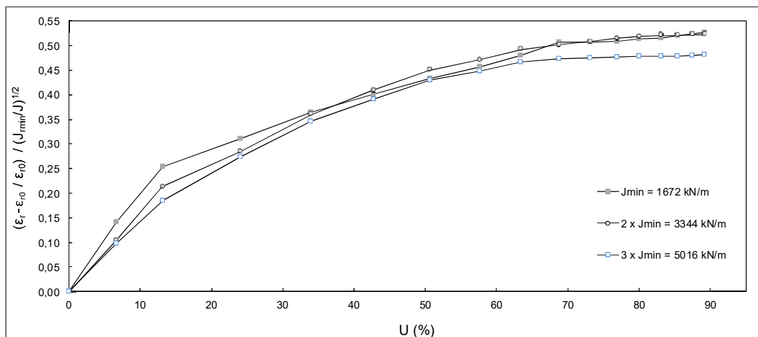
Figure 5. Normalization chart (reinforcement stiffness/strains/ U ).
