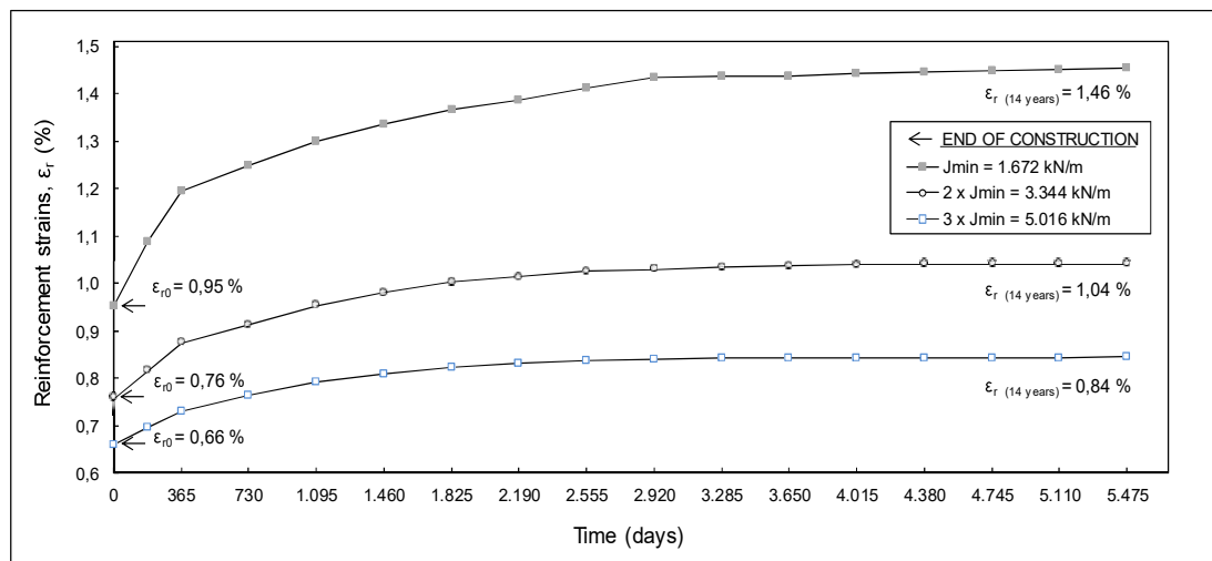
Figure 3. Influence of reinforcement stiffness on mobilized reinforcement strains along the consolidation
