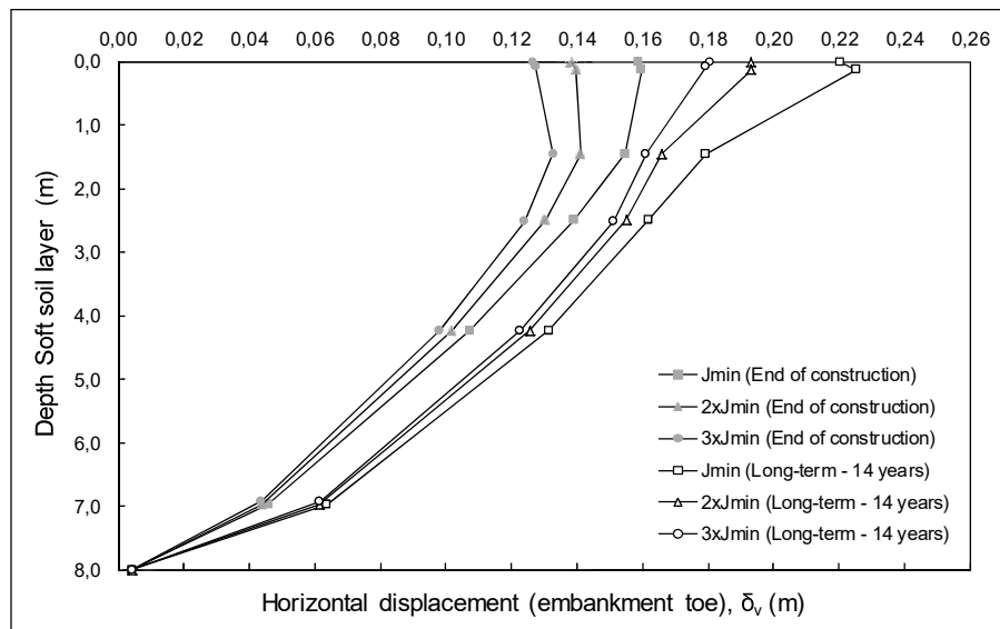
Figure 6. Variation of horizontal displacements with reinforcement stiffness (end of construction and long-term).
