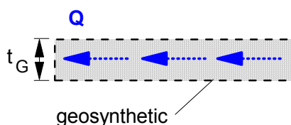
Flow along the geosynthetic plane
